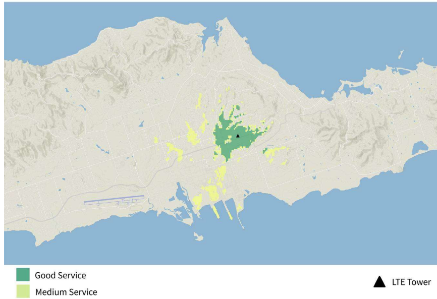
Figure 48. STX-9 TIREM Generated LTE Coverage.
