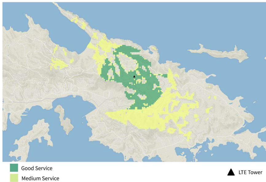
Figure 29. STT-8 TIREM Generated LTE Coverage.
