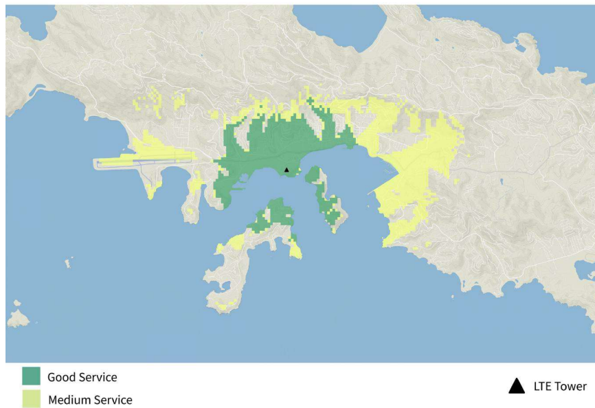
Figure 27. STT-6 TIREM Generated LTE Coverage.
