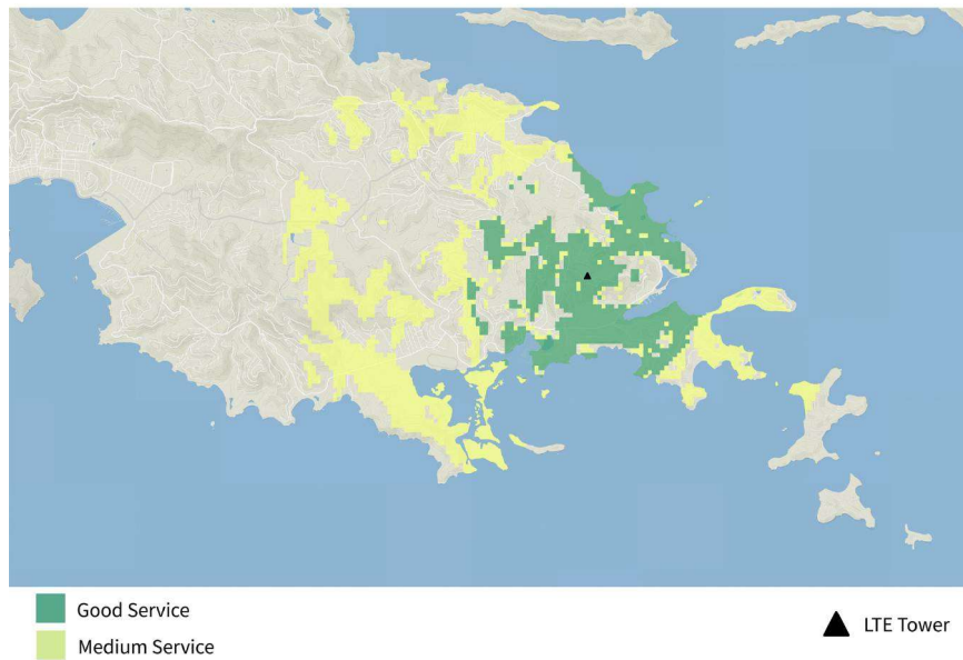
Figure 33. STT-12 TIREM Generated LTE Coverage.
