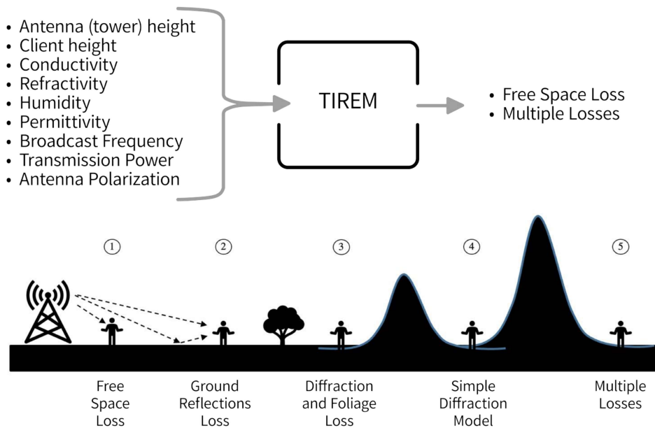
Figure 3. Overview of TIREM, adapted from Wine (2020).
