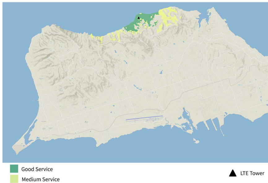
Figure 43. STX-4 TIREM Generated LTE Coverage.
