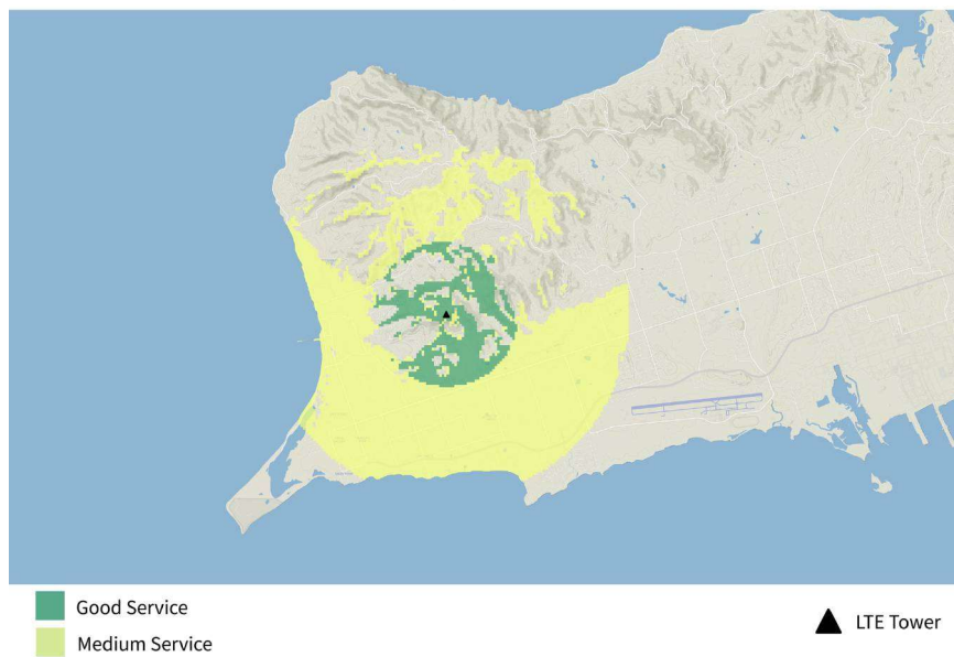
Figure 41. STX-2 TIREM Generated LTE Coverage.
