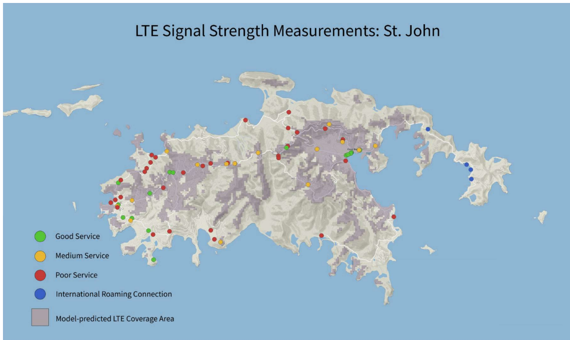
Figure 20. LTE Measurements on STJ along with model-predicted coverage. Measurements were taken primarily along major roads and/or places accessible by personal vehicle.
