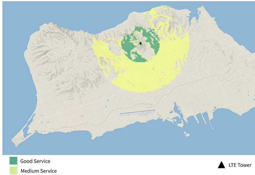
Figure 44. STX-5 TIREM Generated LTE Coverage.
