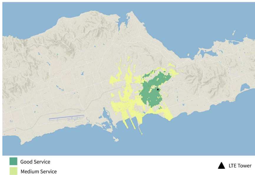
Figure 49. STX-10 TIREM Generated LTE Coverage.
