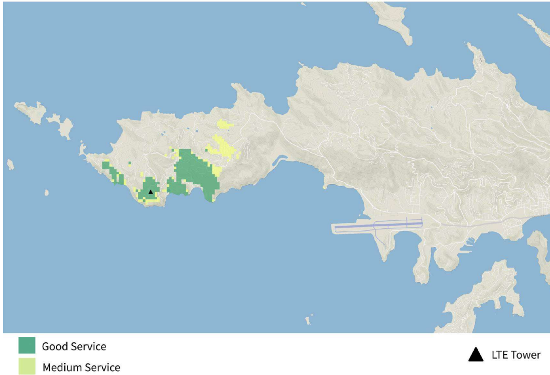
Figure 9. TIREM-Generated LTE Coverage Example for one tower on STT.
