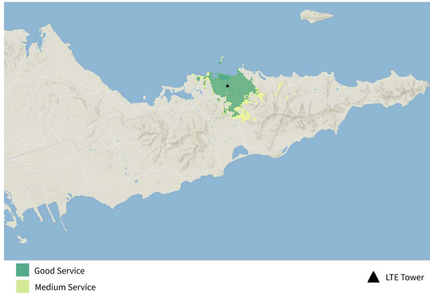
Figure 54. STX-15 TIREM Generated LTE Coverage.
