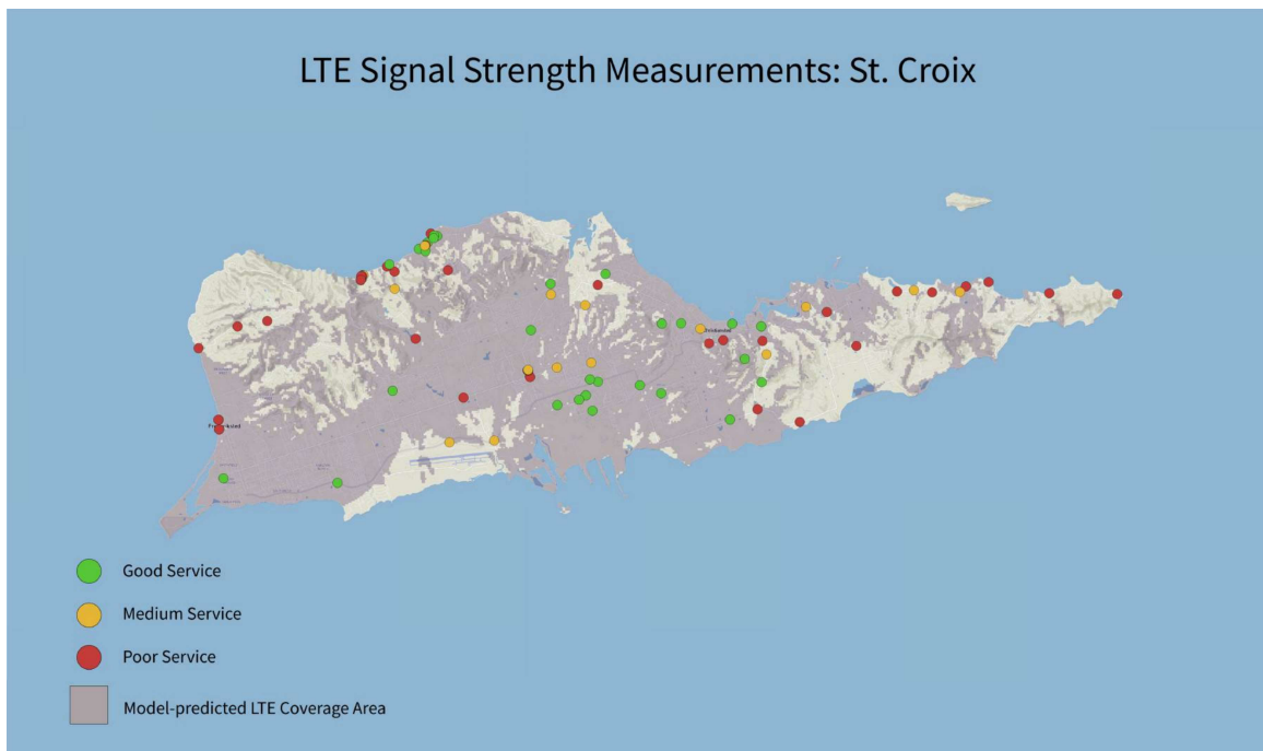
Figure 21. LTE Measurements on STX along with model-predicted coverage. Measurements were taken primarily along major roads and/or places accessible by personal vehicle.
