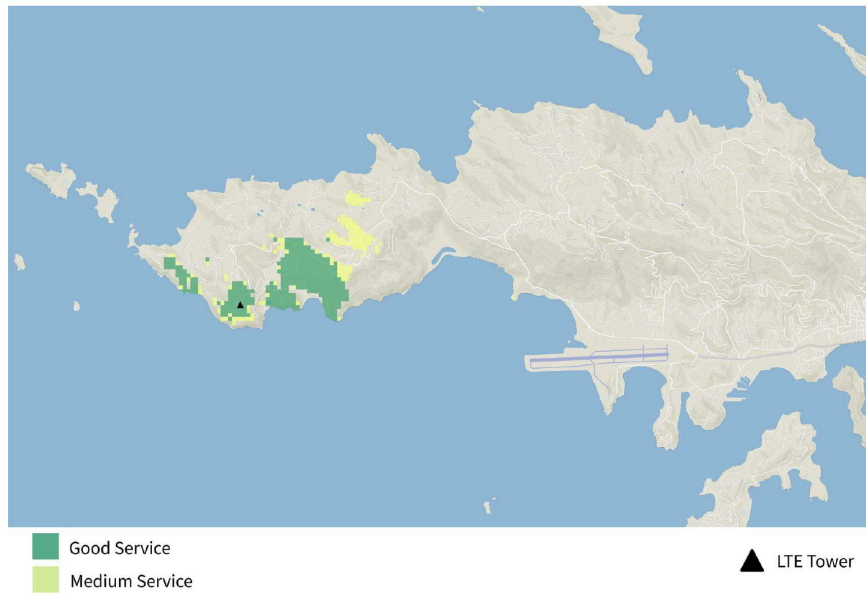
Figure 22. STT-1 TIREM Generated LTE Coverage.
