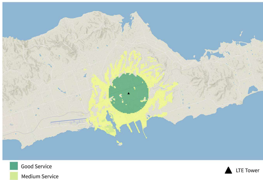
Figure 47. STX-8 TIREM Generated LTE Coverage.
