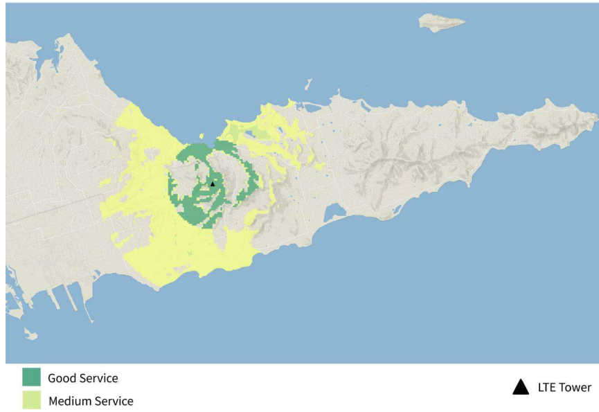
Figure 52. STX-13 TIREM Generated LTE Coverage.
