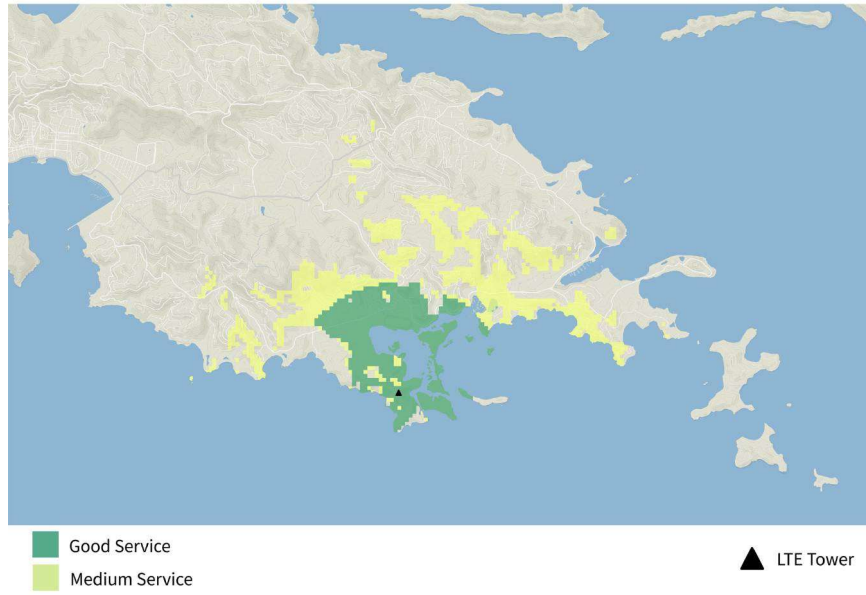
Figure 32. STT-11 TIREM Generated LTE Coverage.
