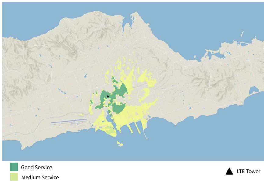
Figure 45. STX-6 TIREM Generated LTE Coverage.
