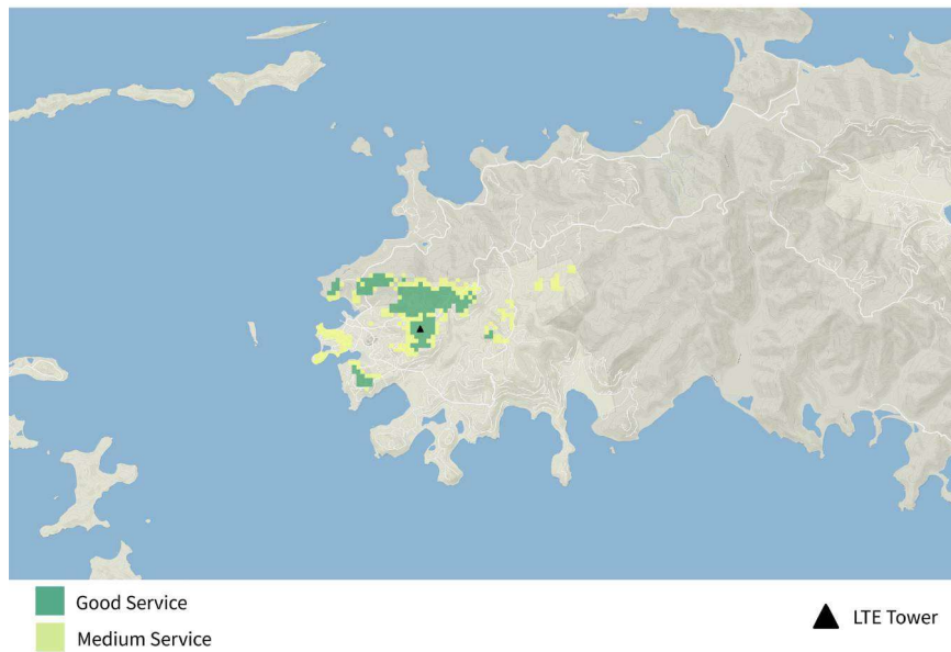
Figure 35. STJ-2 TIREM Generated LTE Coverage.
