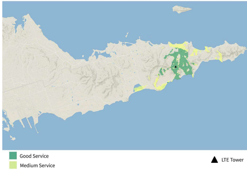
Figure 56. STX-17 TIREM Generated LTE Coverage.
