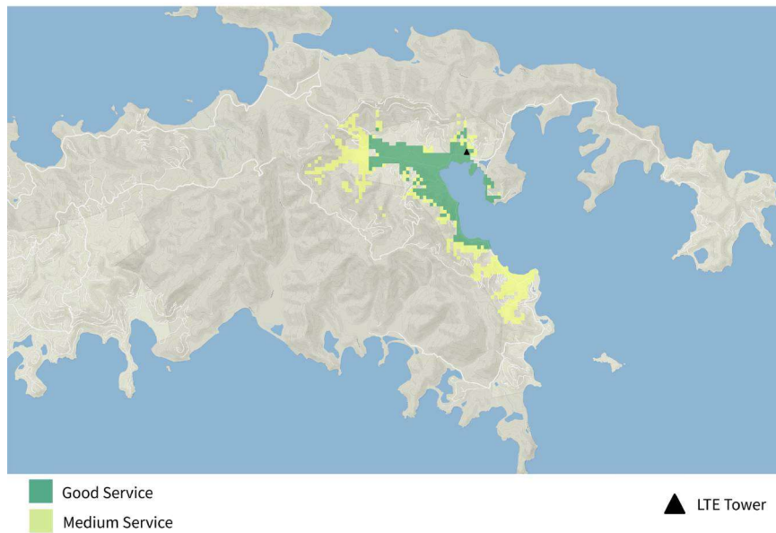
Figure 39. STJ-6 TIREM Generated LTE Coverage.
