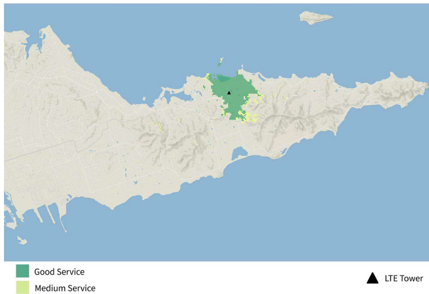
Figure 55. STX-16 TIREM Generated LTE Coverage.
