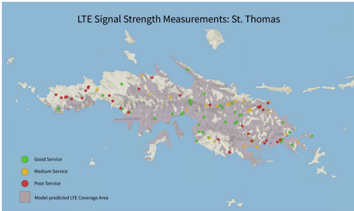
Figure 19. LTE Measurements on STT along with model-predicted coverage. Measurements were taken primarily along major roads and/or places accessible by personal vehicle.
