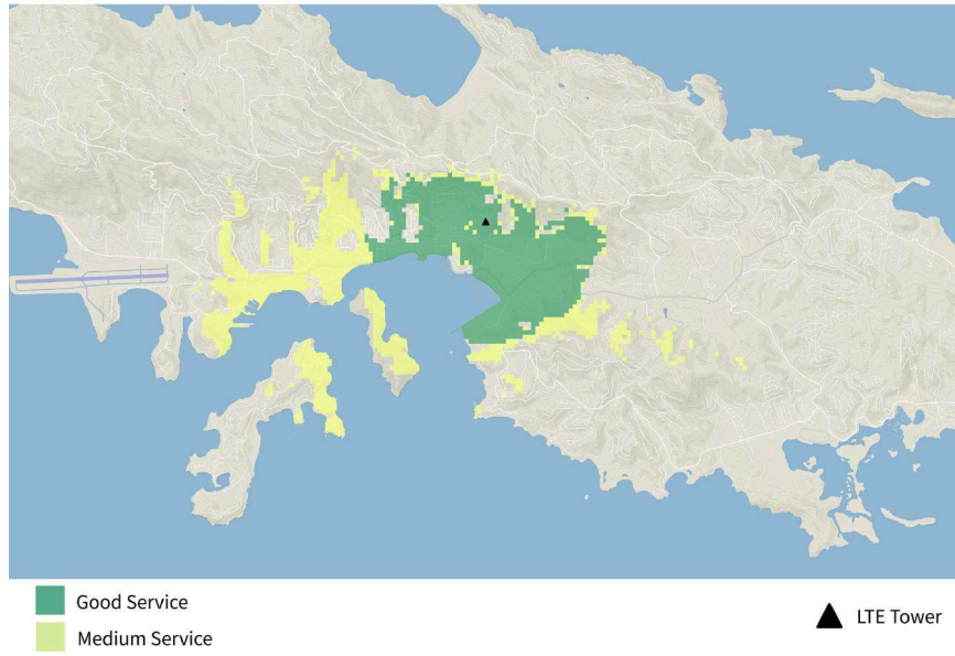
Figure 28. STT-7 TIREM Generated LTE Coverage.
