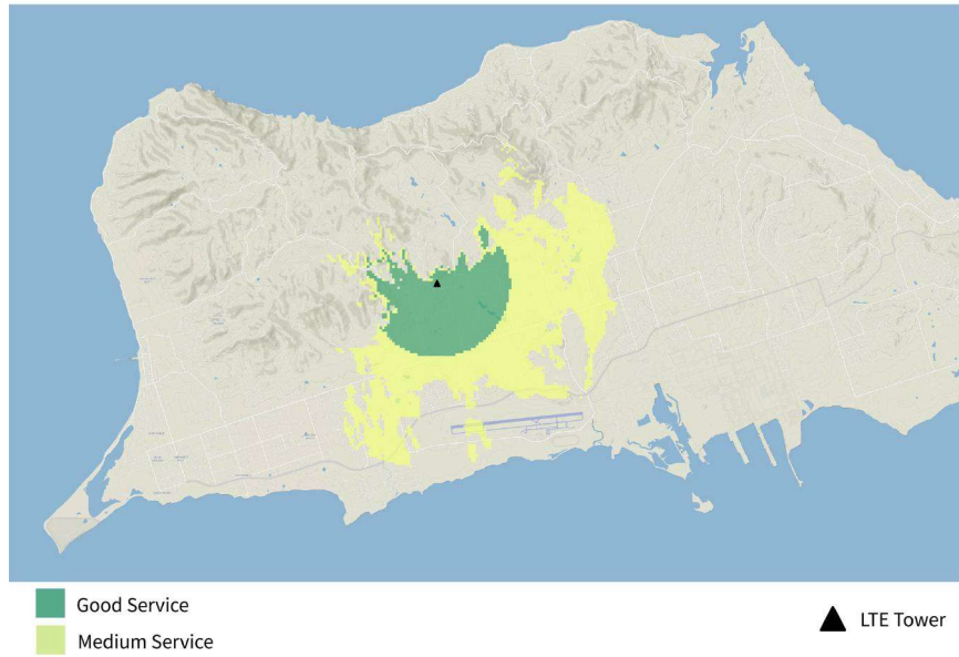
Figure 42. STX-3 TIREM Generated LTE Coverage.
