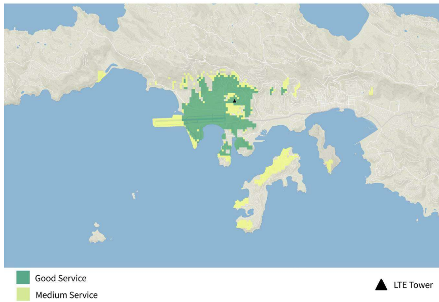
Figure 25. STT-4 TIREM Generated LTE Coverage.
