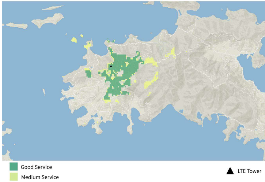
Figure 36. STJ-3 TIREM Generated LTE Coverage.
