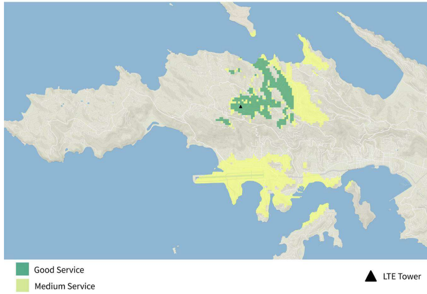
Figure 24. STT-3 TIREM Generated LTE Coverage.
