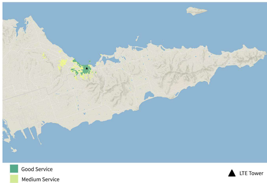
Figure 51. STX-12 TIREM Generated LTE Coverage.
