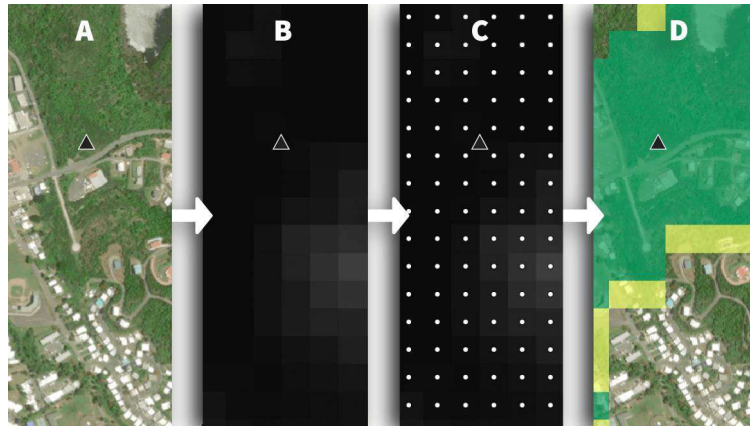
Figure 7. Example of signal raster creation process. A - Identification of tower location, B - elevation raster, C - grid of points created from elevation raster pixel centroids, D - output signal raster with good (green), medium (yellow), and poor (transparent) signal areas identified.
