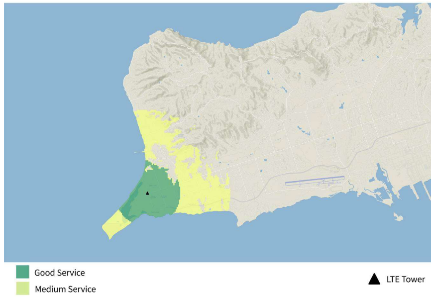
Figure 40. STX-1 TIREM Generated LTE Coverage.
