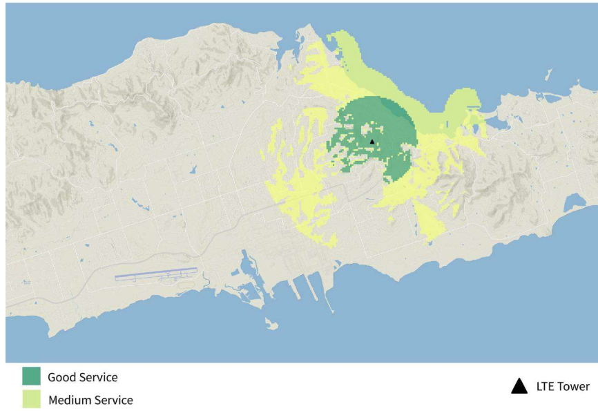
Figure 50. STX-11 TIREM Generated LTE Coverage.
