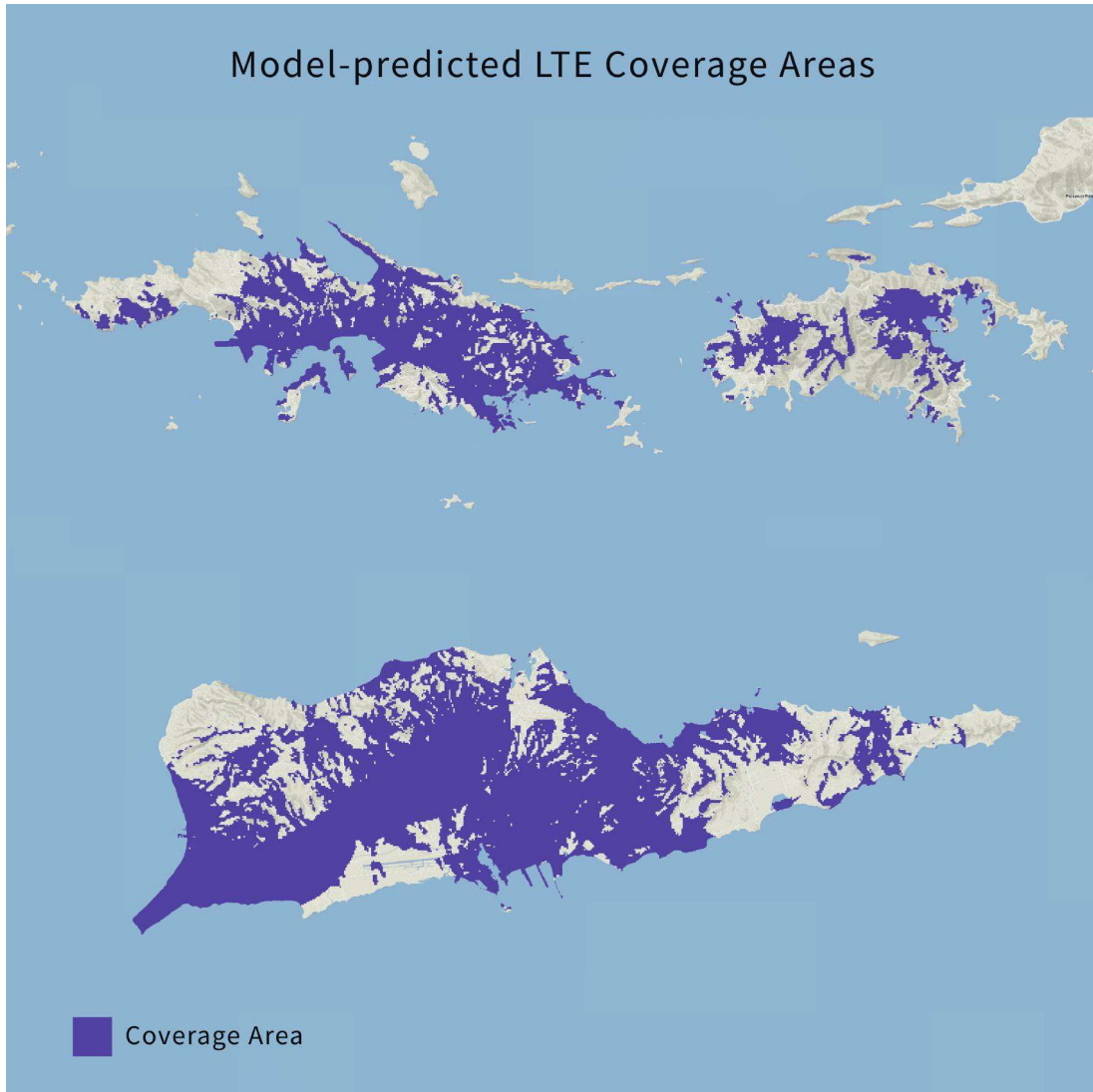
Figure 12. Model-predicted LTE coverage in the USVI. Coverage is defined by an RSRP value of medium service or better. In order to maintain visual consistency with the coverage maps provided by the service providers, any predicted coverage over bodies of water has been omitted from this figure. Note: Distance between the islands is not to scale.
