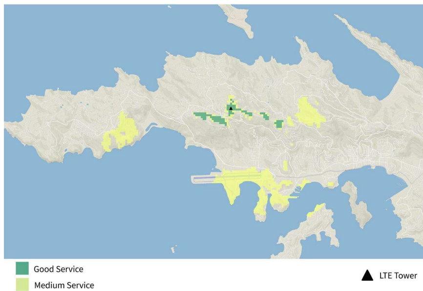
Figure 23. STT-2 TIREM Generated LTE Coverage.
