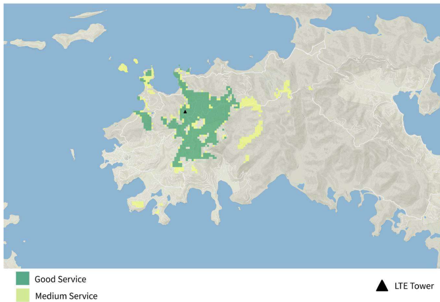
Figure 37. STJ-4 TIREM Generated LTE Coverage.
