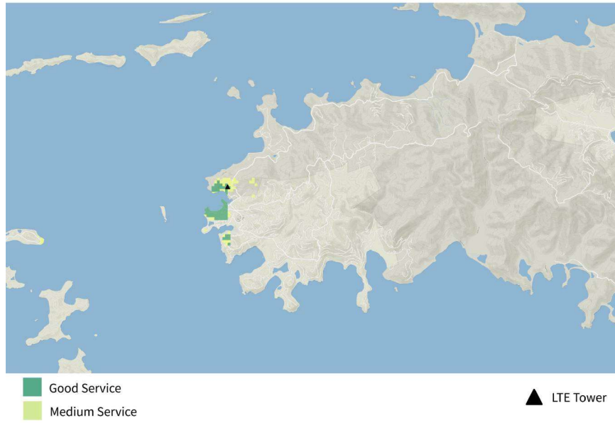
Figure 34. STJ-1 TIREM Generated LTE Coverage.
