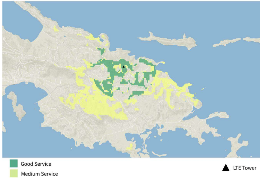
Figure 30. STT-9 TIREM Generated LTE Coverage.
