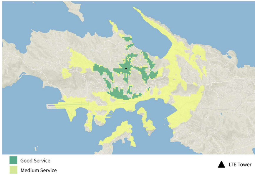
Figure 26. STT-5 TIREM Generated LTE Coverage.
